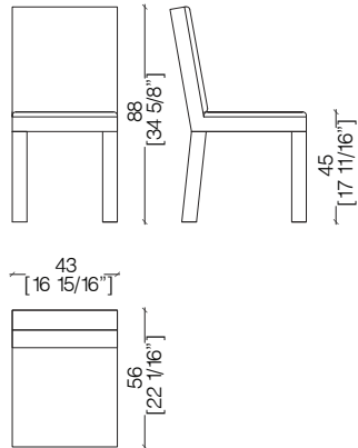
BD 20 chair - sedia - stuhl - chaise - Стул
